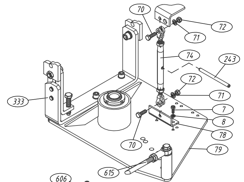
MJT 400 horizontal drive plate
